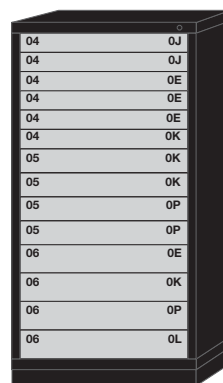
14 drawers with 300 compartments
