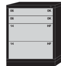
4 drawers with 44 compartments
